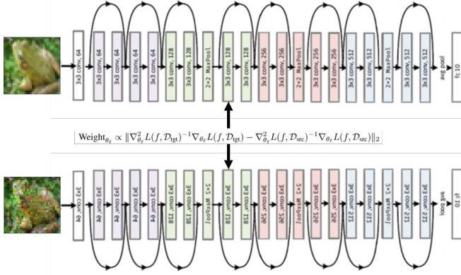
Figure 1: Illustration of AUTO-RGN+HESSIAN+CHANGE
