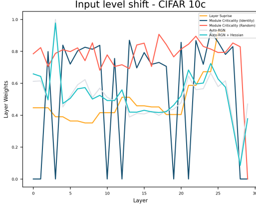
Figure 5: Layer weights for input level shift
