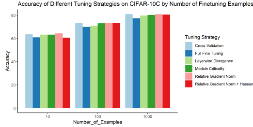
Figure 7: Performance by no. fine-tuning examples
