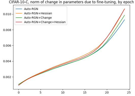
Figure 6: Change in parameters - Auto-RGN
