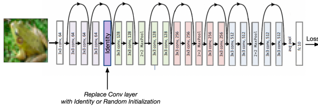
Figure 3: Illustration of MODULE CRITICALITY
