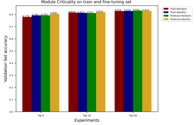
Figure 4: MODULE CRITICALITY hyperparameter investigation
