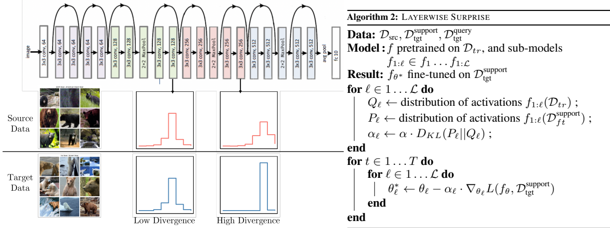
Figure 2: Illustration of LAYERWISE SURPRISE
