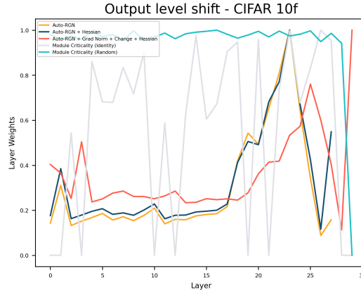
Figure 9: Layer weights for output level shift
